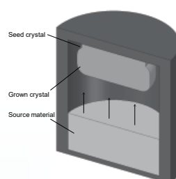
Vapor growth method
