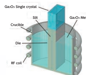
Melt growth method
